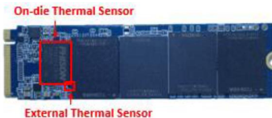
Figure 2-1 Thermal Sensor
